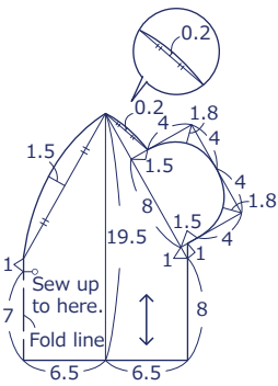
Baby Cap Outer piece Outer fabric x 2
