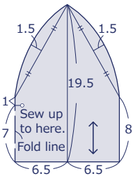
Baby Cap Lining piece Lining fabric x 2
